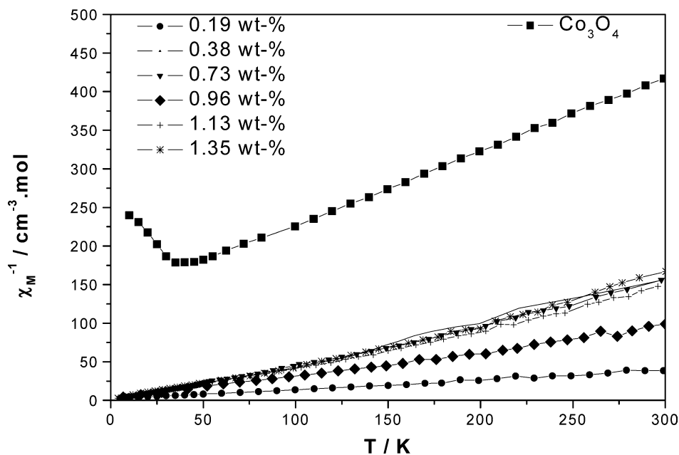
Fig. 3. Temperature dependence of the reciprocal susceptibility of catalysts (the curve of \text{Co}_3\text{O}_4 is also shown for comparison).
